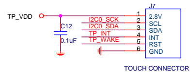
TOUCH CONNECTOR
