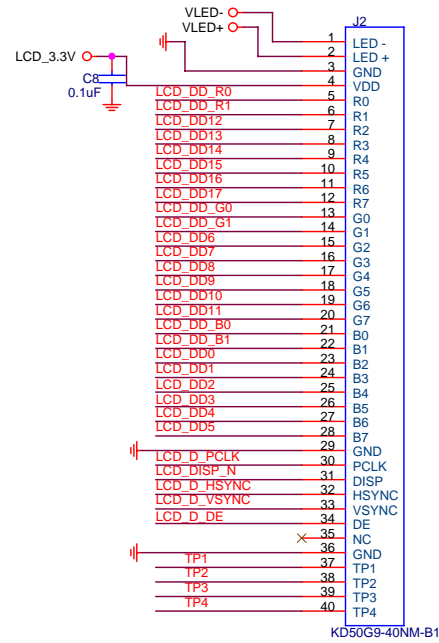
KD50G9-40NM-B1
