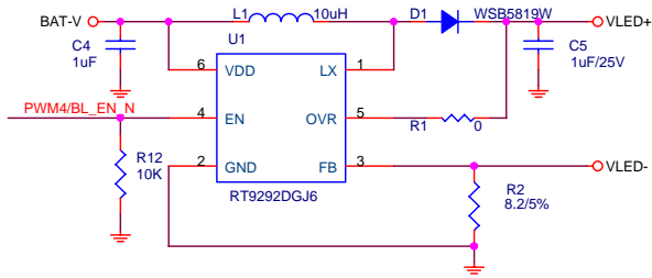
LCD BackLight
