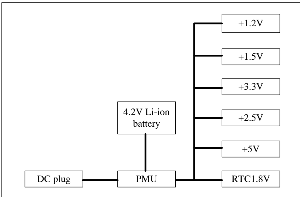
Figure 16-1 Power Architecture
