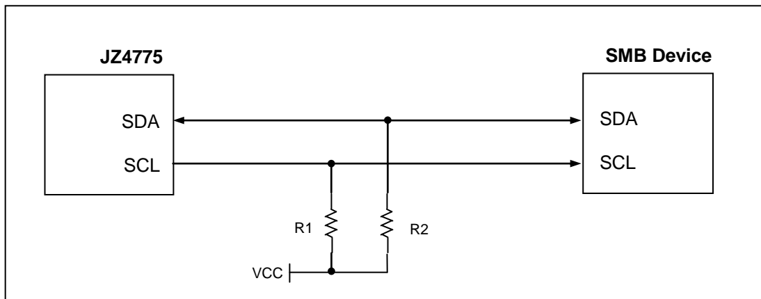
Figure 14-5 SMB Interconnection
