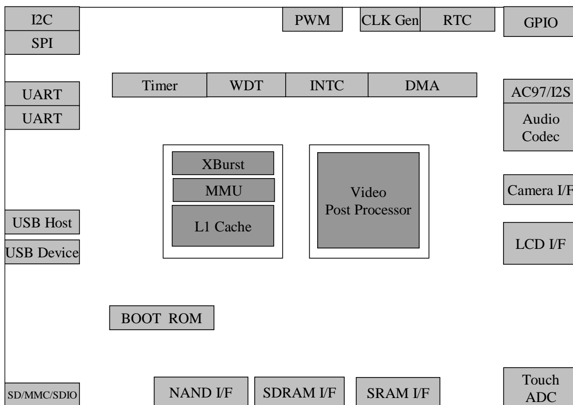
Figure 1-1 Jz4740 Diagram
