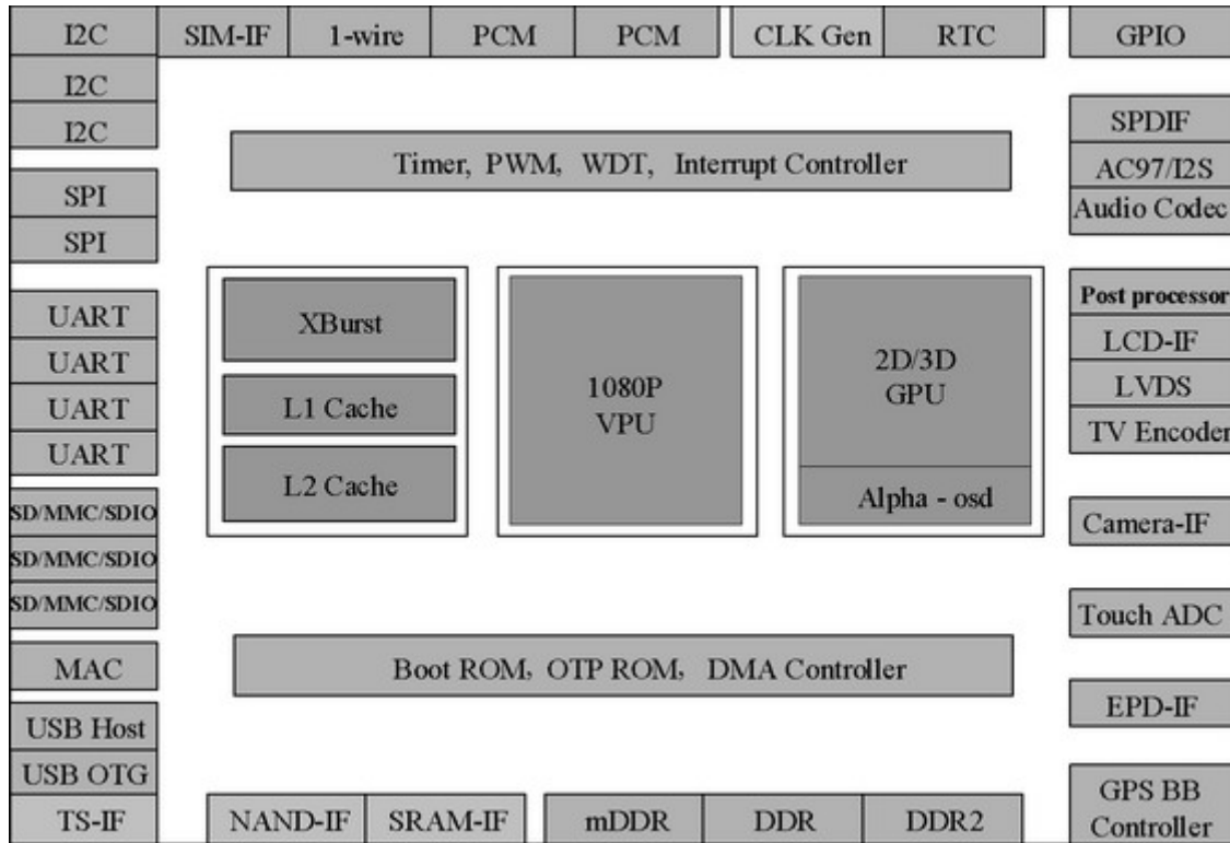
Figure 1-1 JZ4770 Diagram
