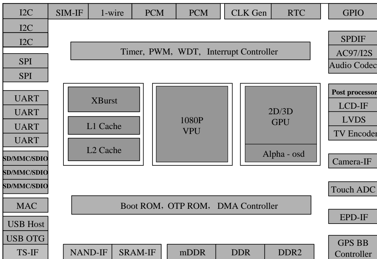
Figure 1-1 JZ4770 Diagram
