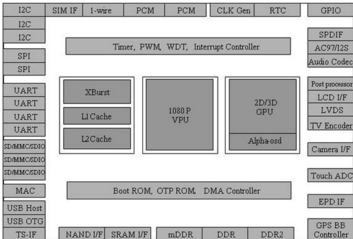
Figure 1-1 JZ4770 Diagram
