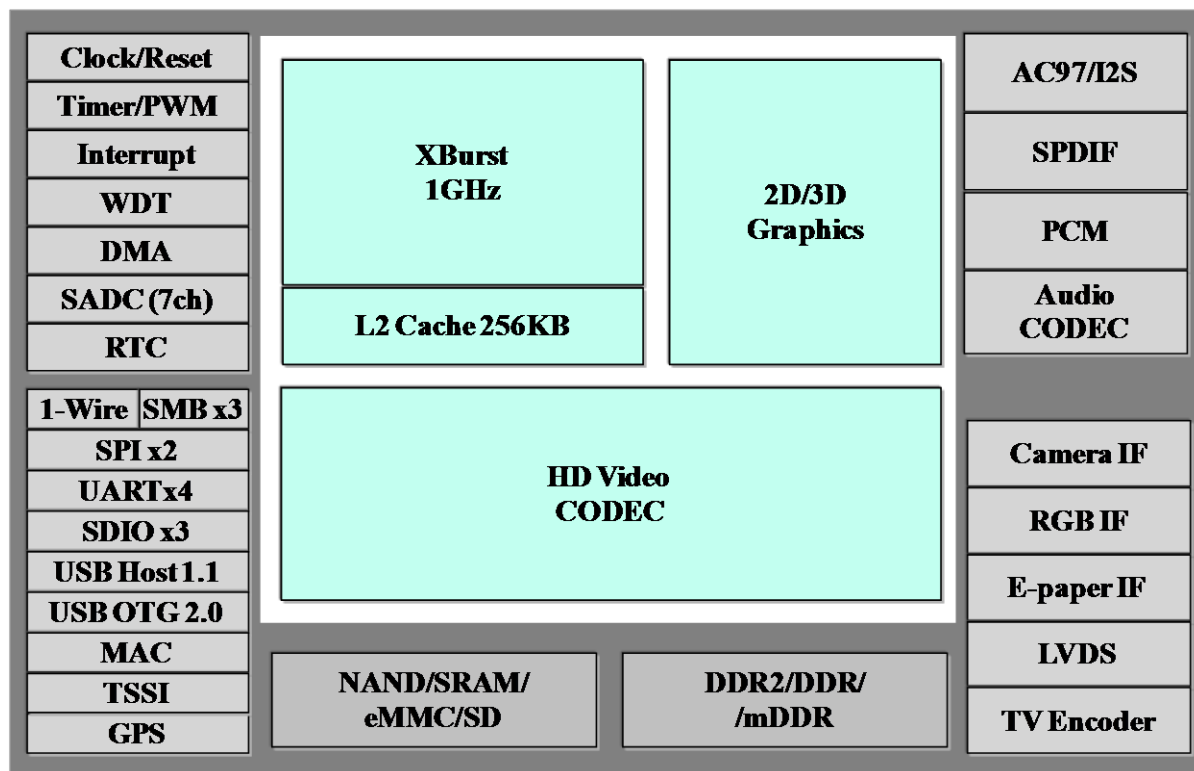
Figure 1-1 JZ4770 Diagram
