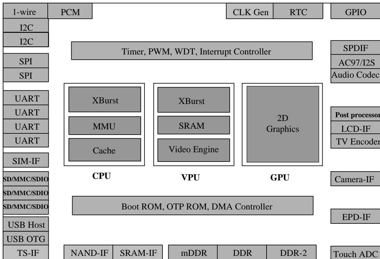
Figure 1-1 JZ4760 Diagram
