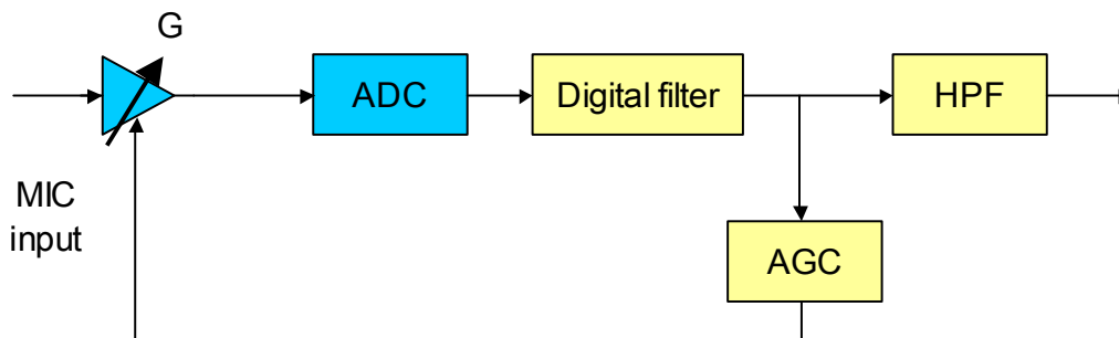
Figure 19-6 AGC Function Block Diagram
