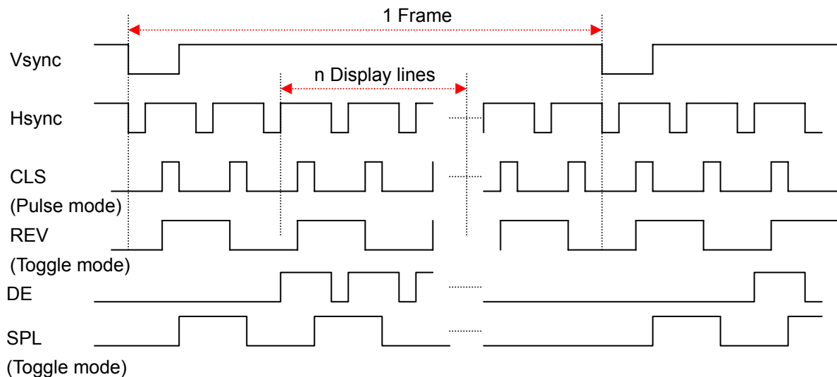
Figure 14-11 Special TFT LCD Timing 2
