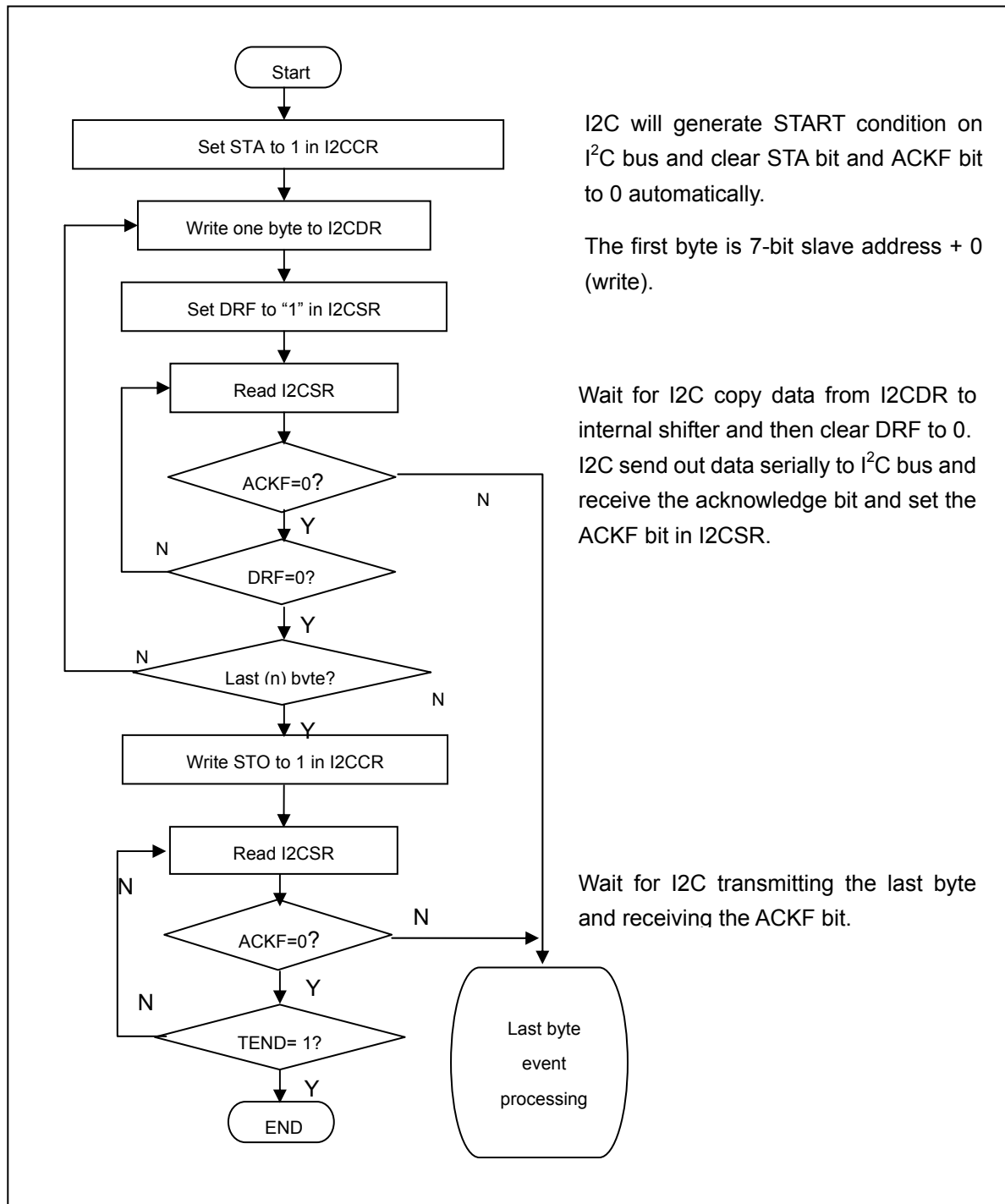
Figure 23-9 I2C Write Operation Flowchart
