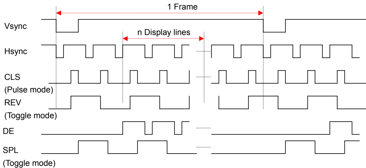
Figure 14-10 Special TFT LCD Timing 1
