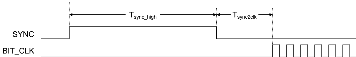
Figure 20-11 Warm AC '97 CODEC Reset Timing
