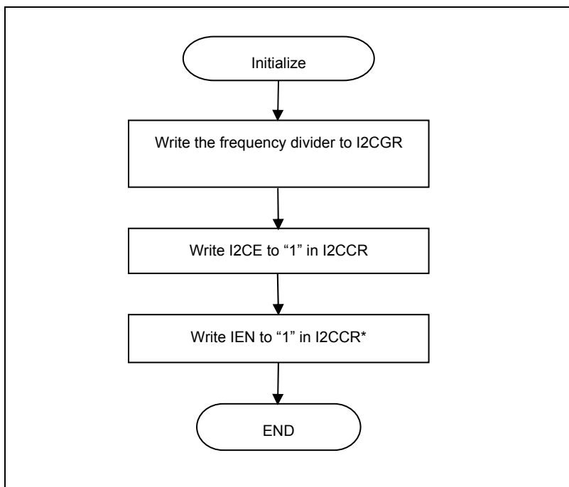
Figure 23-8 I2C Initialization
