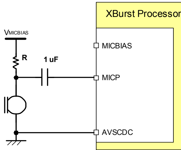
Figure 19-16 MIC connection with external V_{MICBIAS}
