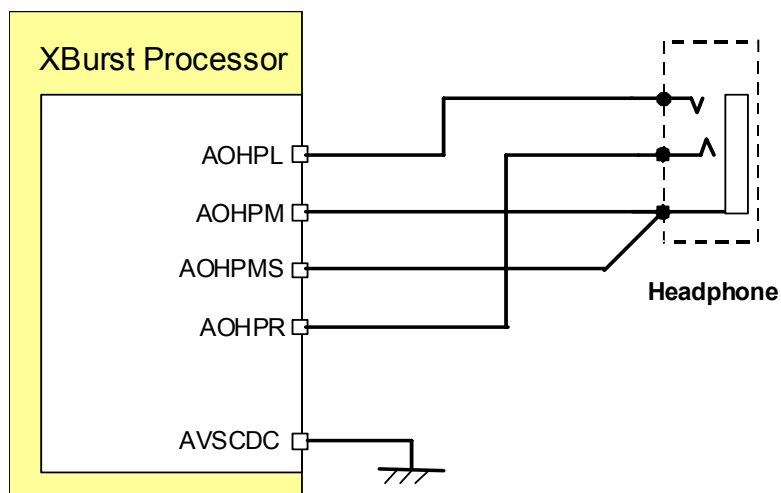
Figure 19-13 Capacitor-less connection
