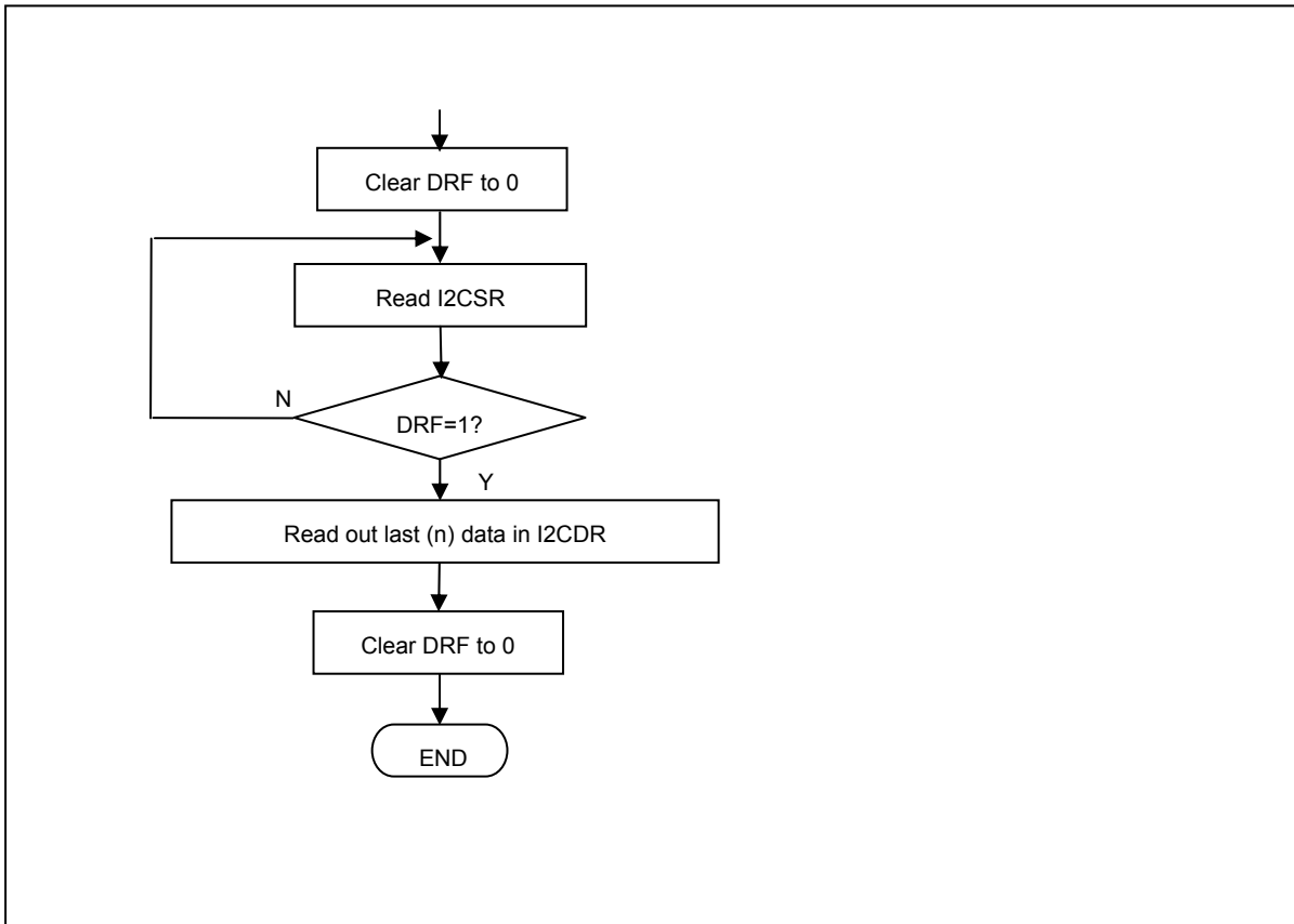
Figure 23-11 Read Operation Flowchart (cont.)
