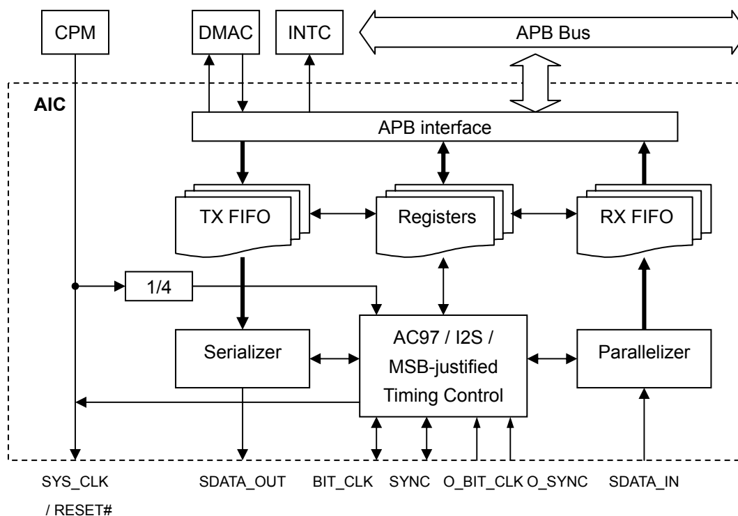
Figure 20-1 AIC Block Diagram
