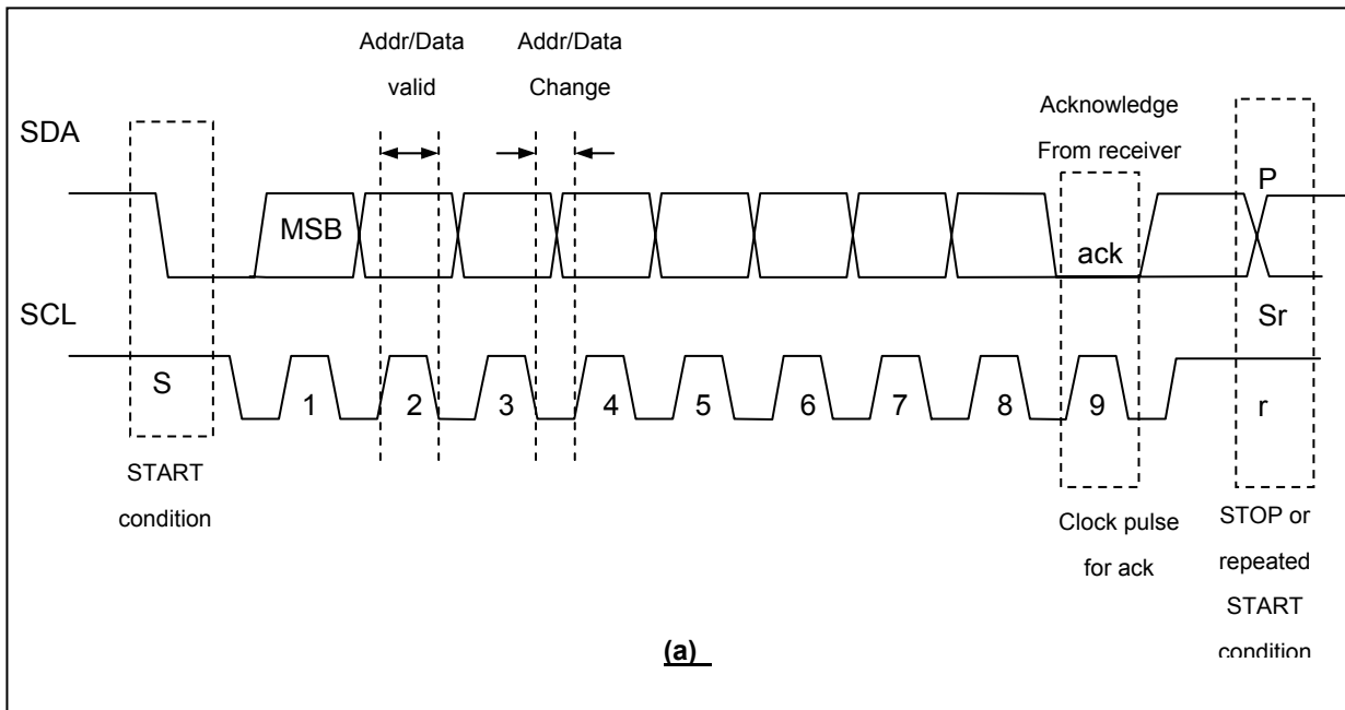
Figure 23-1 I2C-bus Protocol
