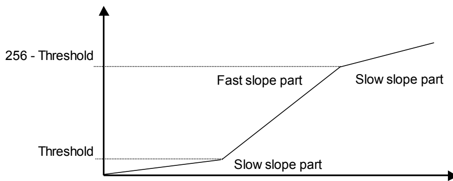
Figure 19-5 Ramp up
