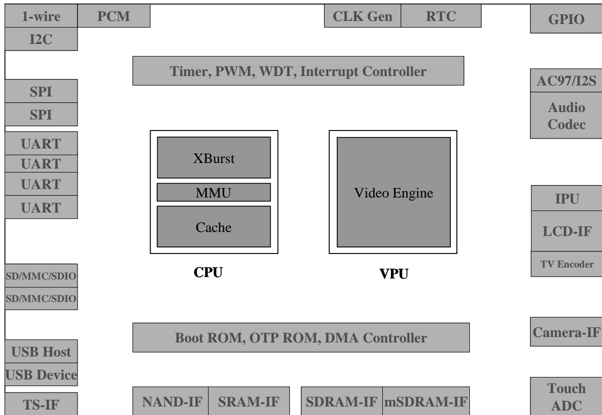
Figure 1-1 JZ4750 Diagram
