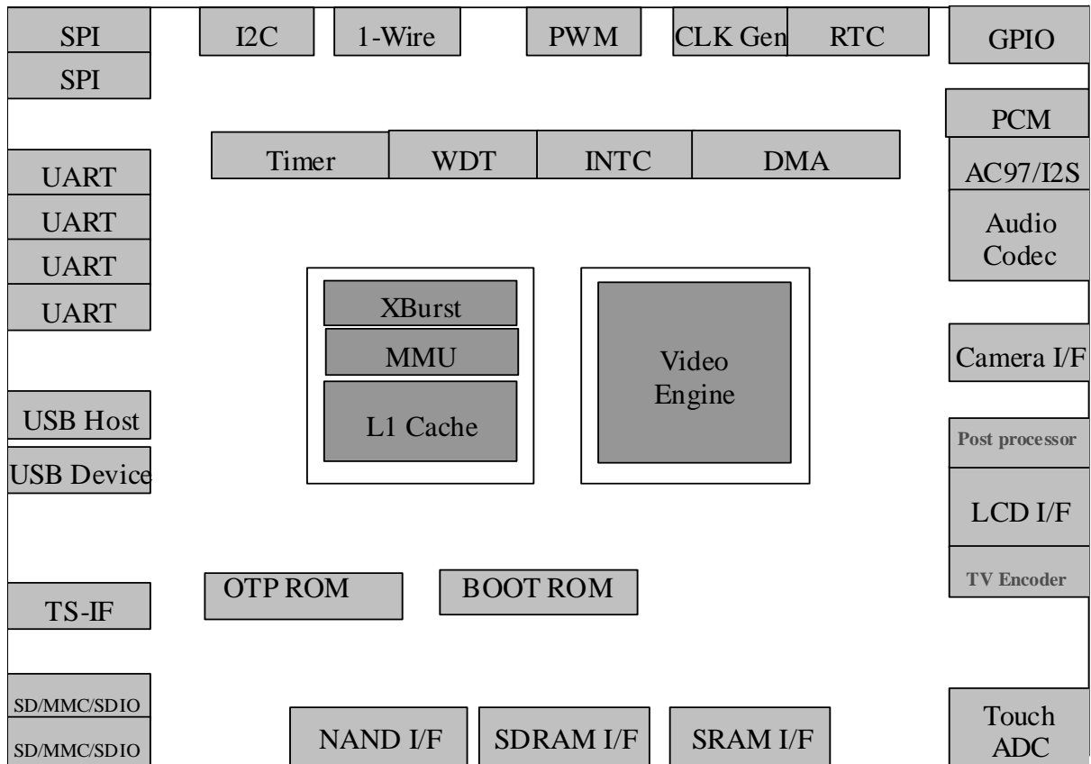
Figure 1-1 JZ4750 Diagram
