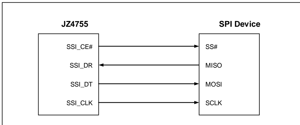
Figure 11-3 SPI Interconnection
