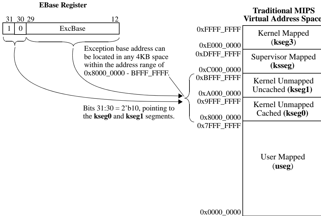
Figure 3.40 Location of Exception Vector Base Address in Traditional MIPS Virtual Address Space
