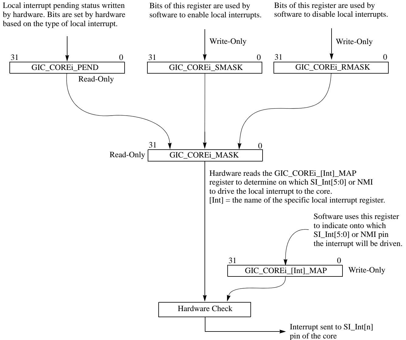
Figure 12.7 Local Interrupt Masking and Mapping in the GIC
