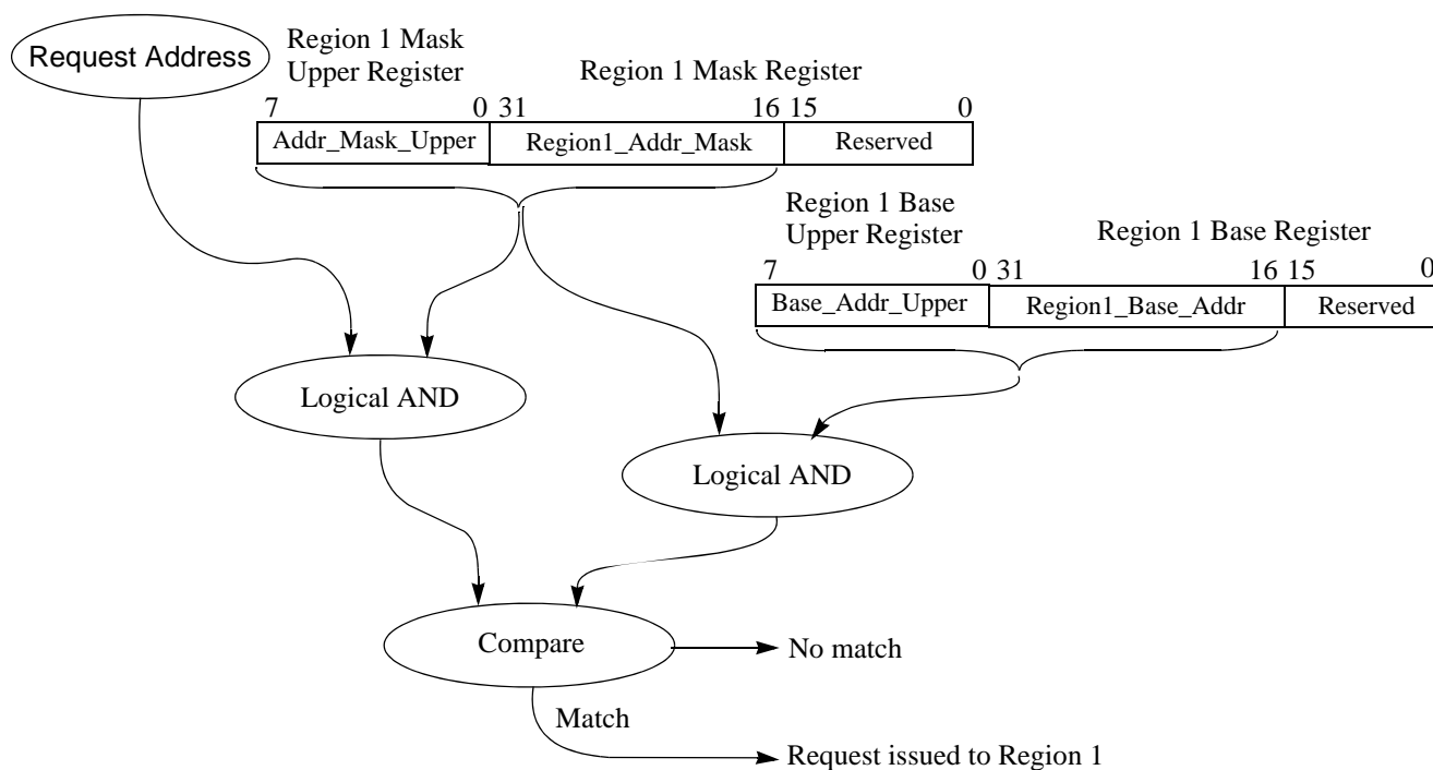
Figure 11.5 Mapping a Request to Region 1 in XPA Mode
