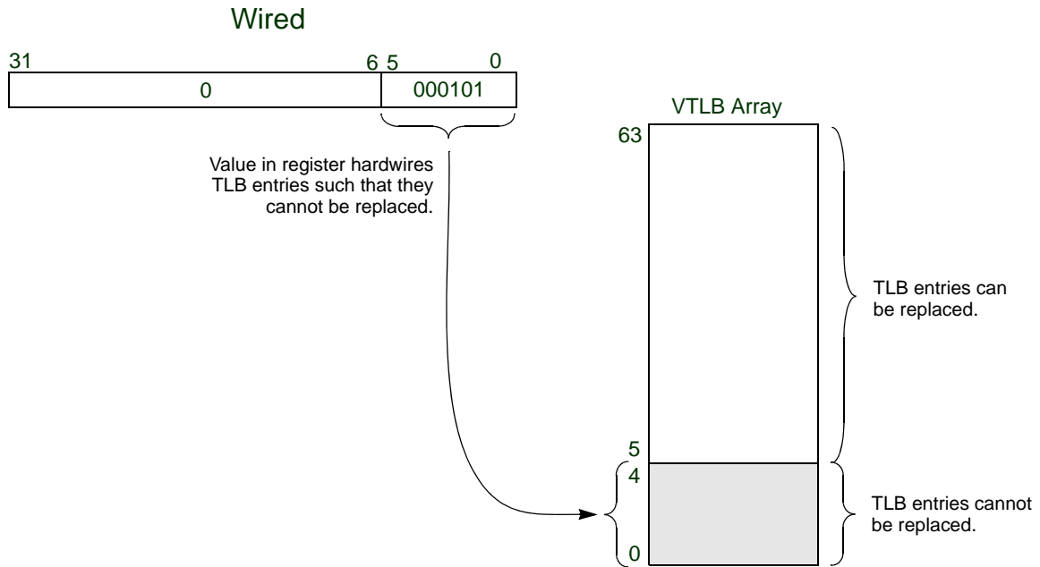
Figure 3.34 Hardwiring Entries in the VTLB
