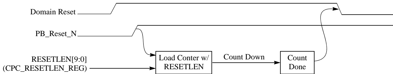
Figure 10.3 Extending the Reset Sequence Beyond the Assertion of the Reset Signal
