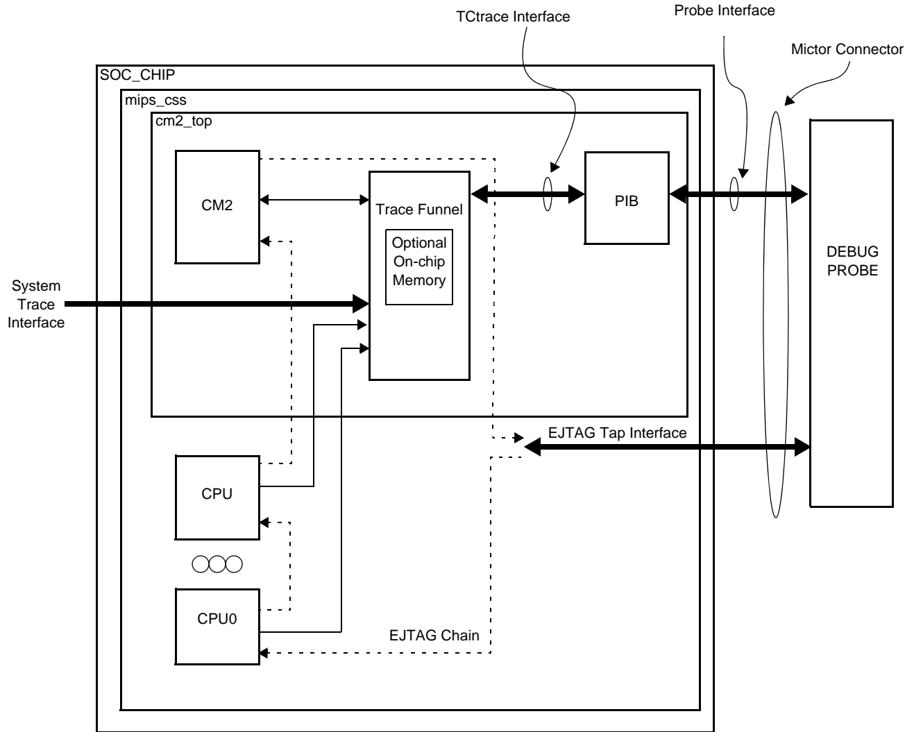
Figure 15.1 Trace Connections in the MIPS Debug Architecture
