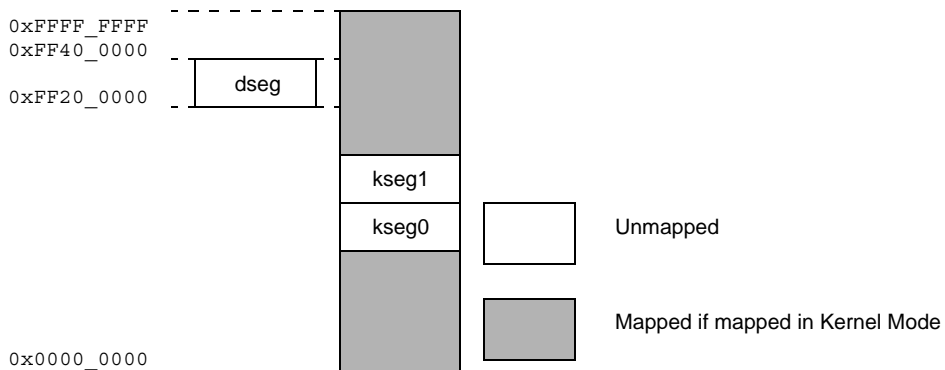
Figure 3.50 Debug Mode Virtual Address Space
