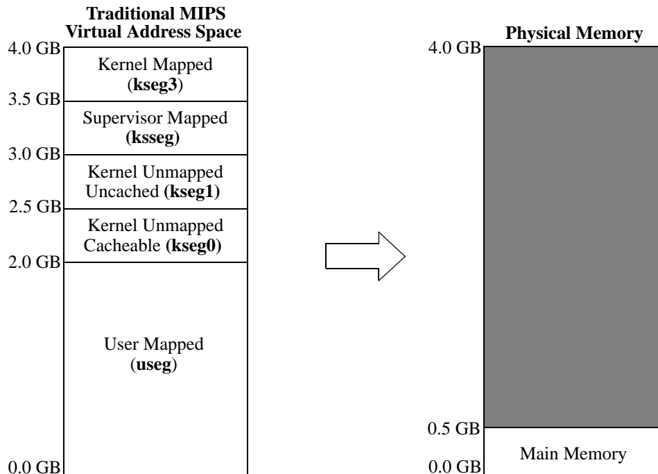
Figure 3.13 Traditional Virtual Address Mapping in Previous Generation MIPS32 Processors
