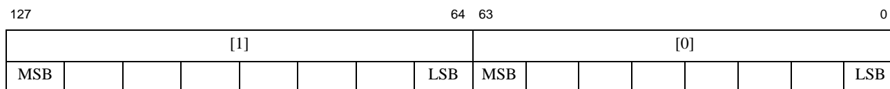
Figure 14.5 MSA Vector Register Doubleword Elements
