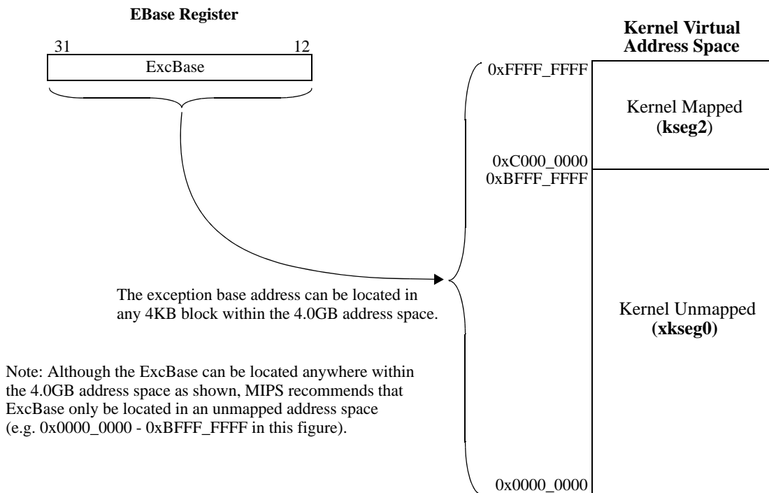
Figure 3.41 Location of Exception Vector Base Address Using the Enhanced Virtual Addressing Scheme
