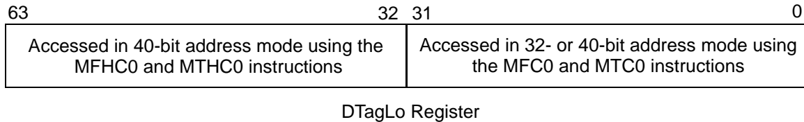
Figure 2.46 Accessing the 64-bit DTagLo Register
