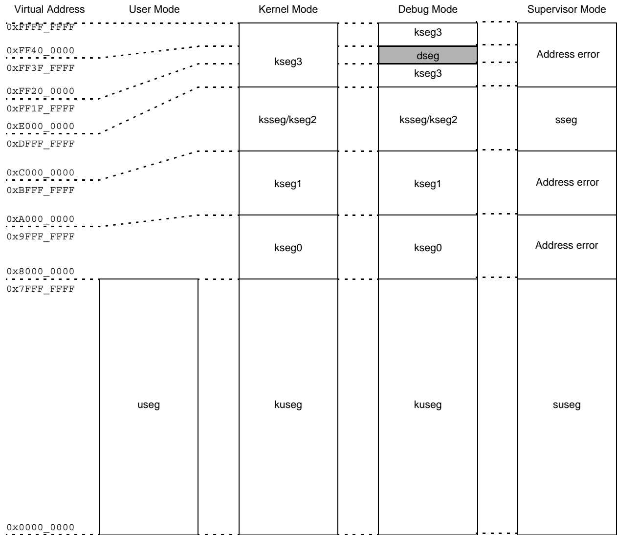
Figure 3.42 Virtual Memory Map — Legacy Mode
