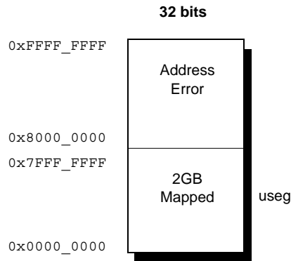
Figure 3.44 User Mode Virtual Address Space — Legacy Configuration
