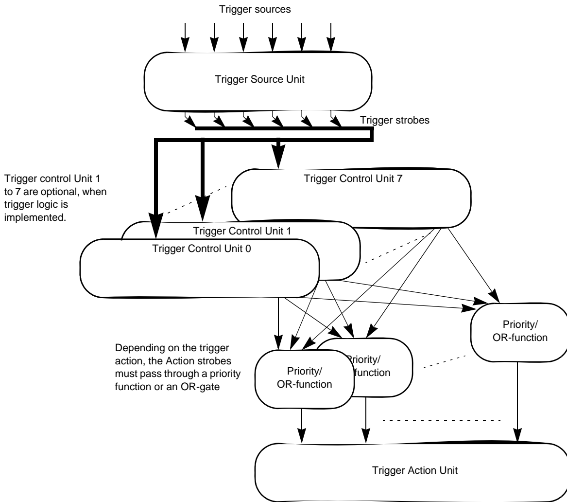
Figure 15.41 TCB Trigger Processing Overview
