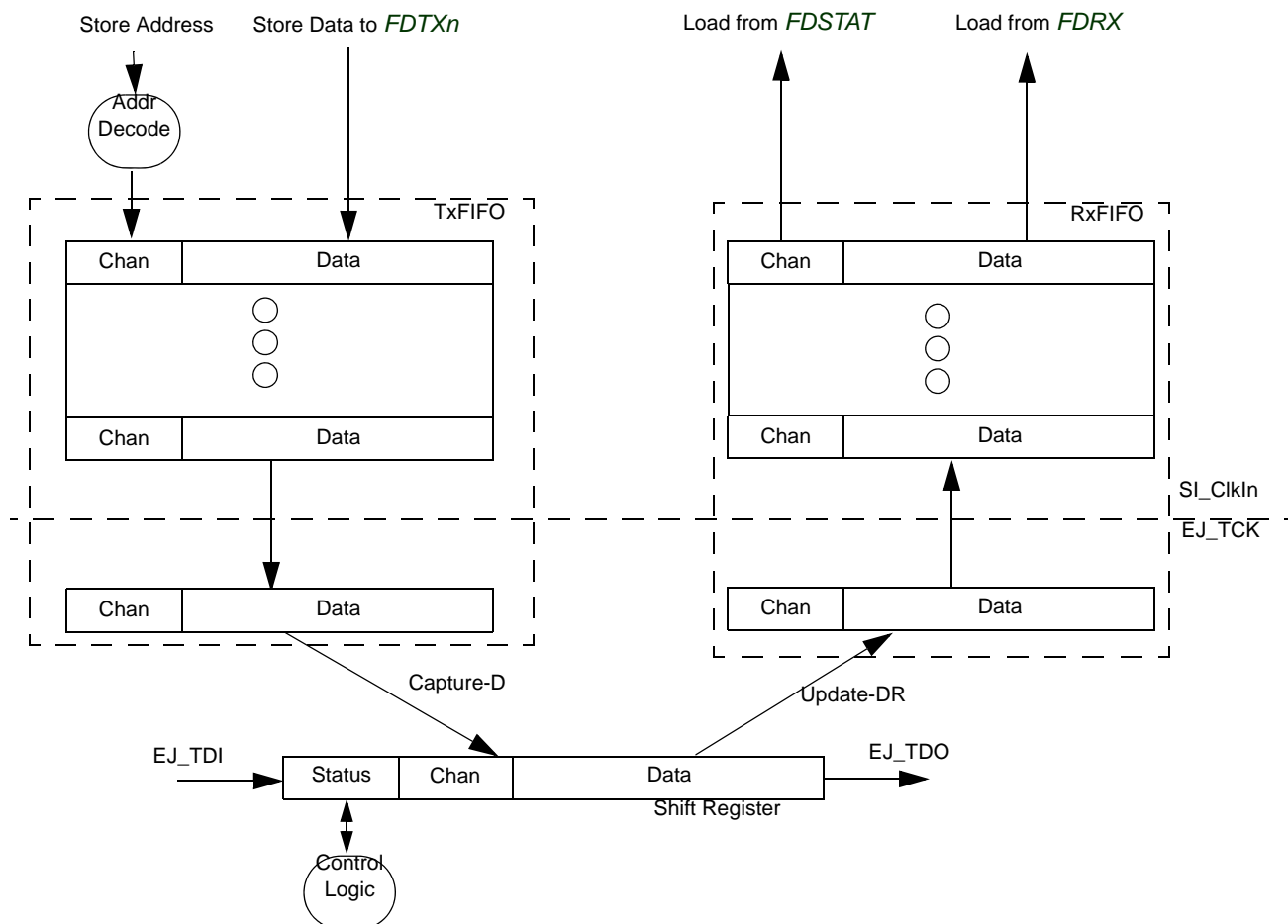
Figure 15.40 Fast Debug Channel Buffer Organization
