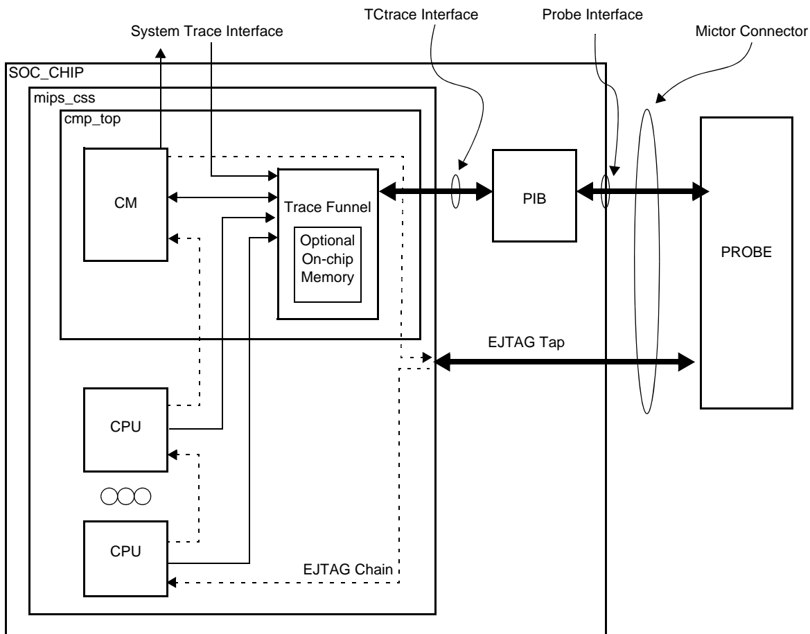
Figure 16.1 PD Trace Architecture
