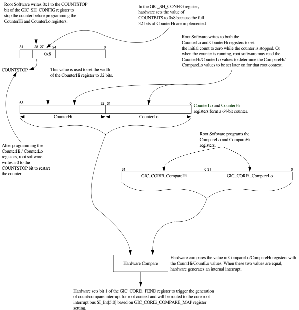
Figure 12.11 Root Context Count-Compare Timer Interrupt Generation Flow
