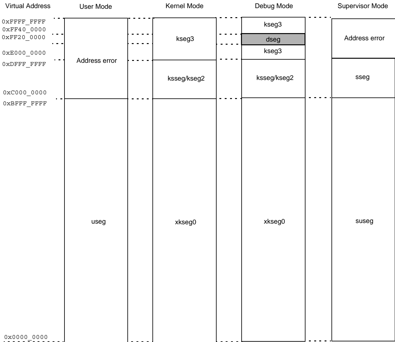
Figure 3.43 Virtual Memory Map — EVA Mode, 3GB xkseg0 Example
