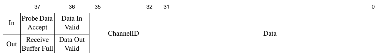
Figure 15.26 FDC TAP Register Format
