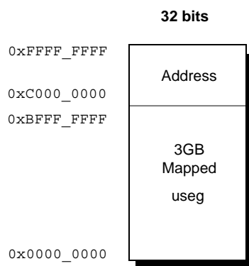
Figure 3.45 User Mode Virtual Address Space — EVA Mode
