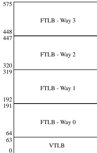
Figure 3.2 P5600 VTLB and FTLB
