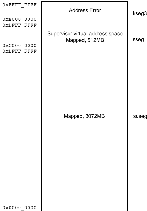
Figure 3.47 Supervisor Mode Virtual Address Space — EVA Configuration
