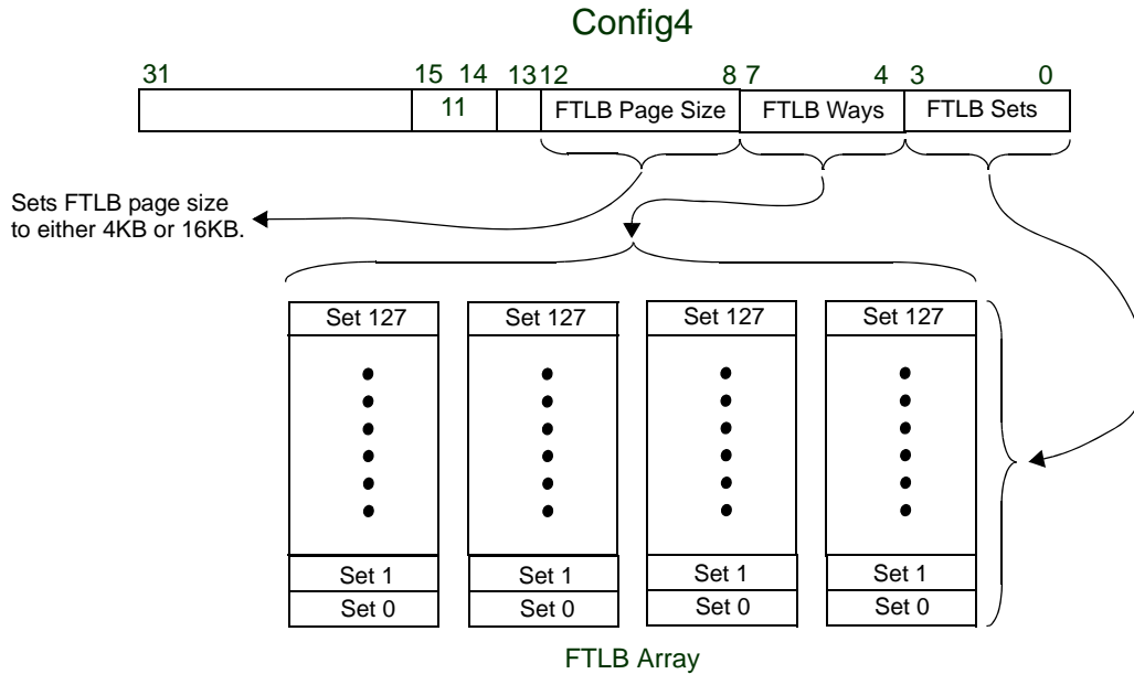
Figure 3.5 Determining the FTLB Characteristics — FTLB Present and Enabled
