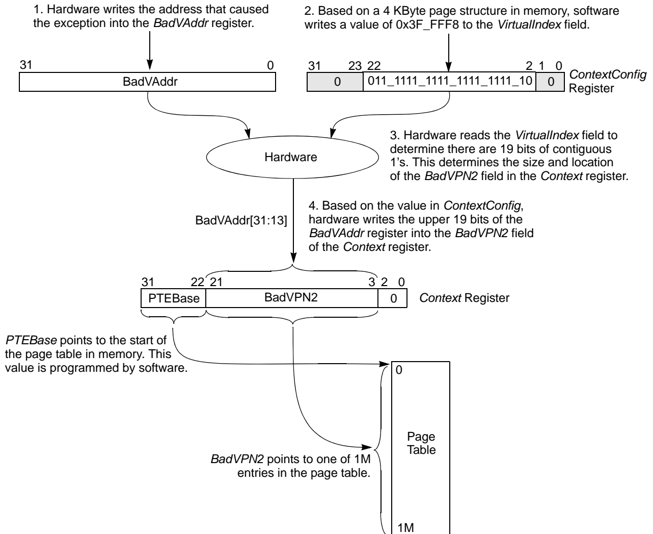
Figure 3.38 TLB Exception Flow Example — Single Level Table, 4 KB Page Size
