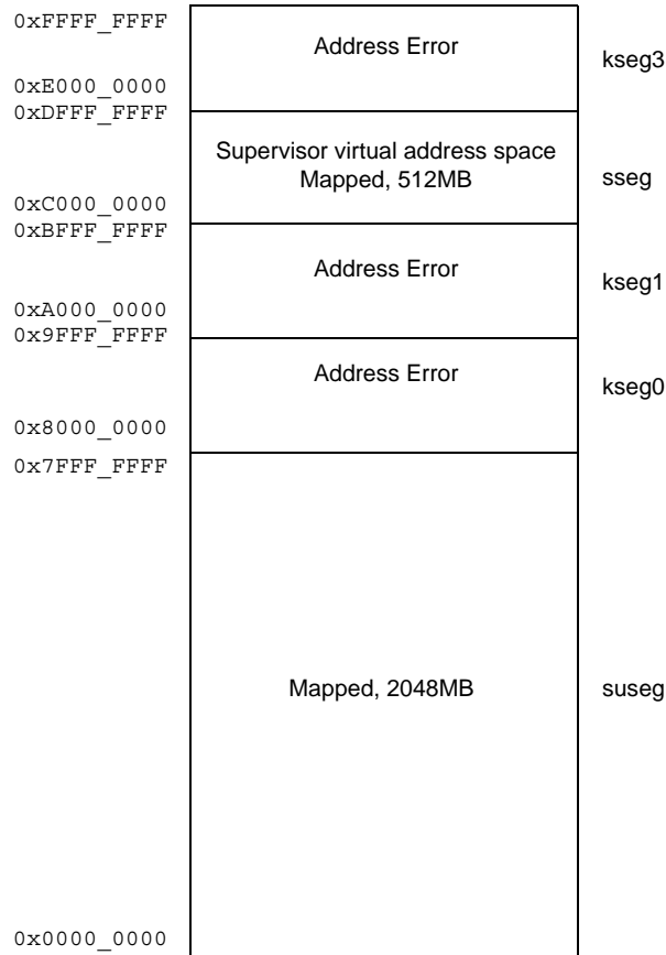
Figure 3.46 Supervisor Mode Virtual Address Space
