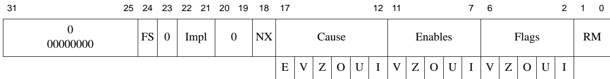
Figure 14-33 MSACSR Register Format
