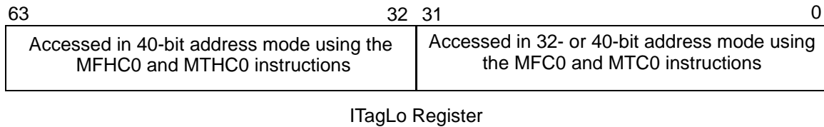
Figure 2.40 Accessing the 64-bit ITagLo Register
