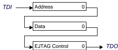
Figure 15.3 Concatenation of the EJTAG Address, Data and Control Registers
