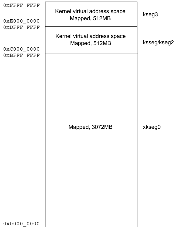
Figure 3.49 Kernel Mode Virtual Address Space — EVA Mode, 3GB Example
