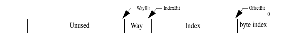
Figure 17.2 Usage of Address Fields to Select Index and Way
