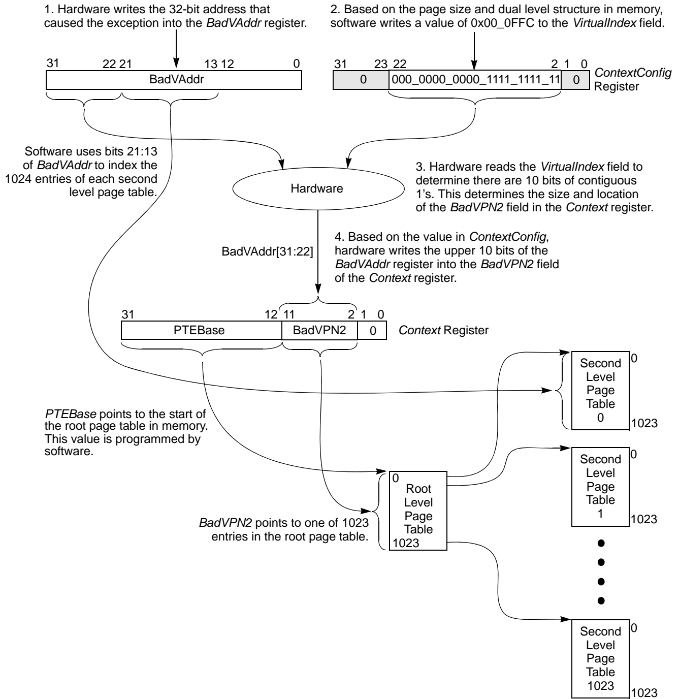
Figure 3.39 TLB Exception Flow Example — Dual Level Table, 4 KB Page Size
