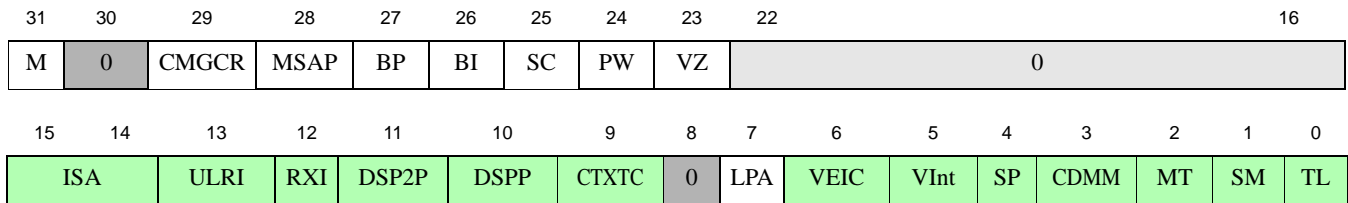
Figure 2.5 Config3 Register Format
