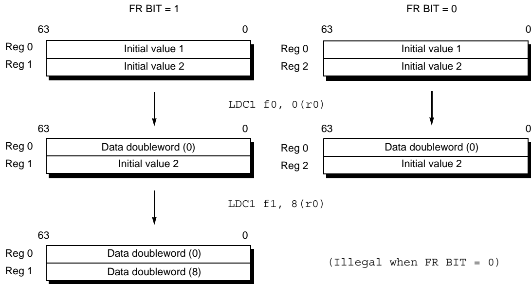
Figure 14.24 FPU Doubleword Load and Move-to Operations
