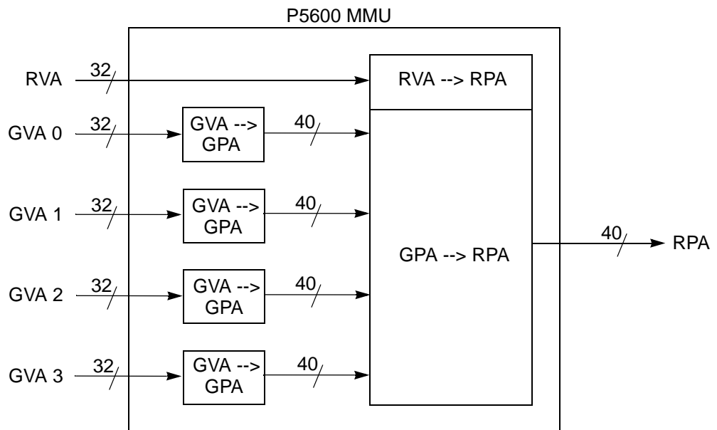
Figure 5.1 Overview of XPA Translation Process
