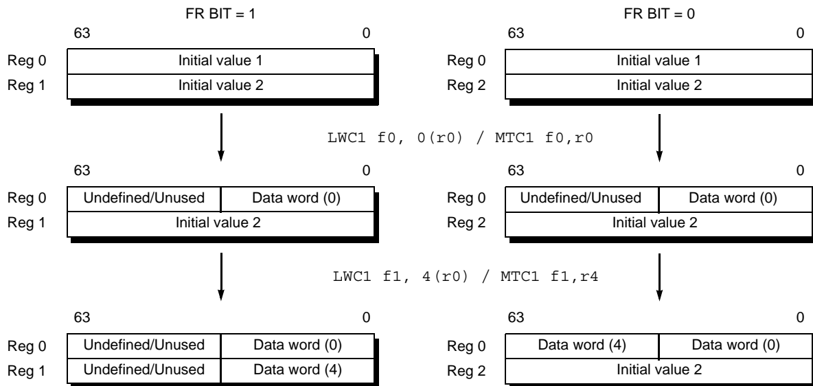
Figure 14.23 FPU Word Load and Move-to Operations
