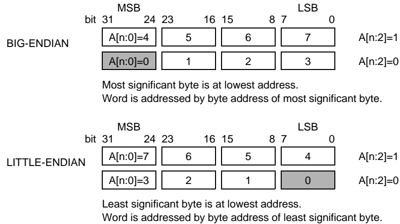
Figure 15.24 Endian Formats for the Data Register
