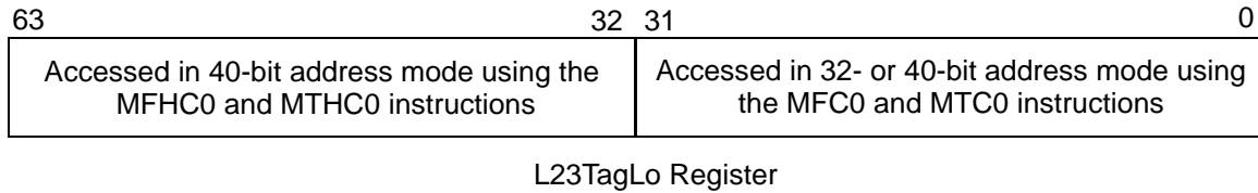
Figure 2.51 Accessing the 64-bit L23TagLo Register
